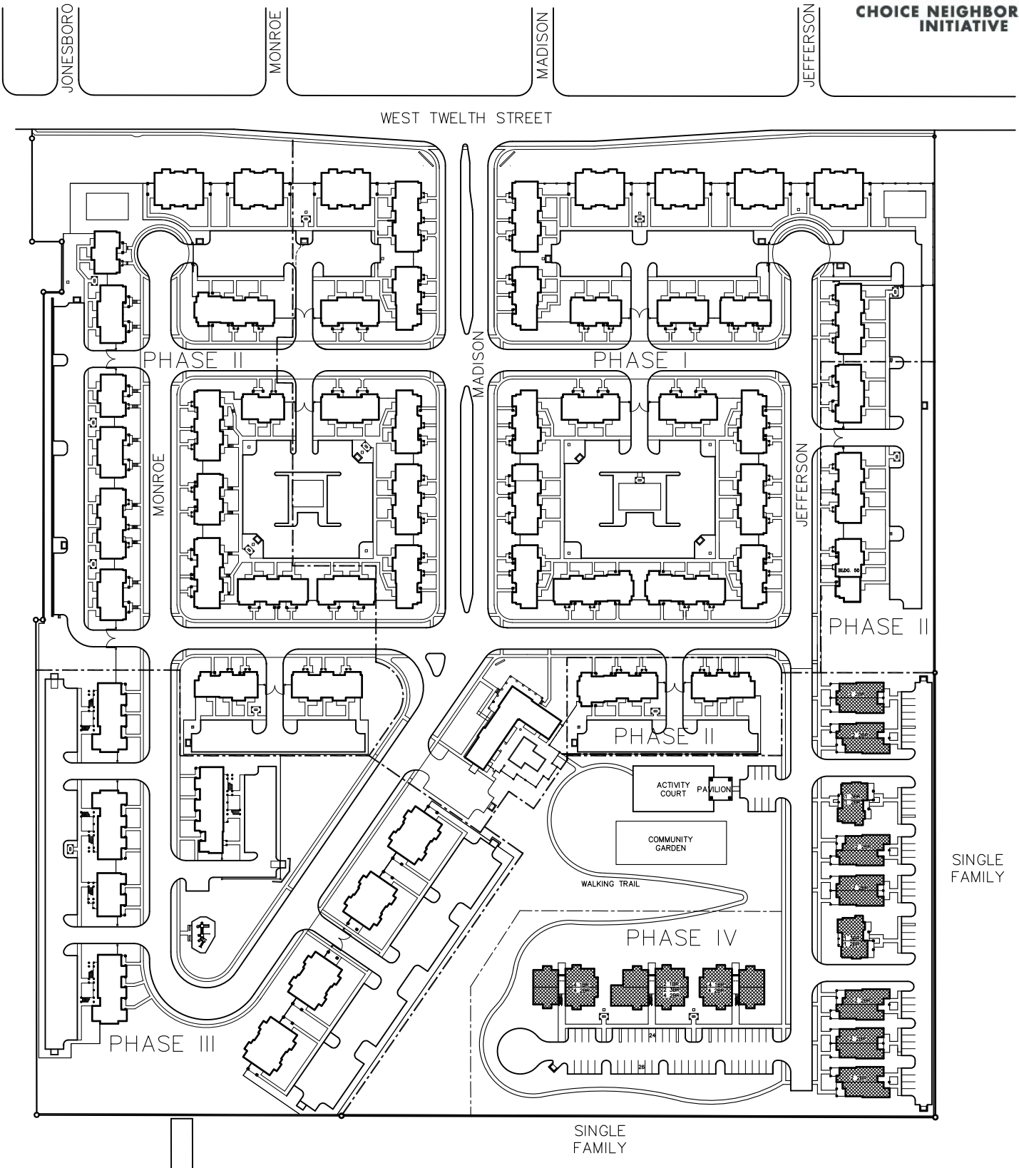
PROPOSED SITE PLAN 1" = 180' - 0"
